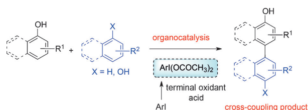
Scheme 1. The metal-free organocatalytic oxidative cross-coupling of phenols by hypervalent iodine catalyst.
